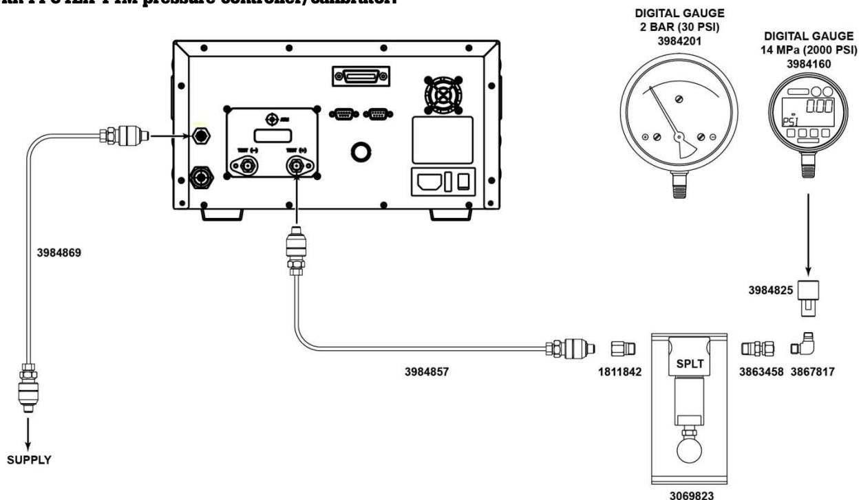
Figure 1: 14 MPa PPC4E Demo Kit Assembly
