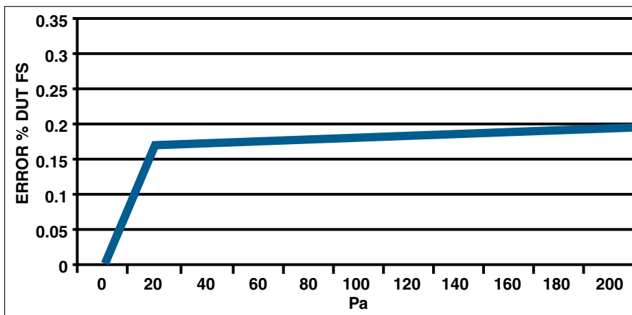
Figure 3. Error caused by poor zero.
