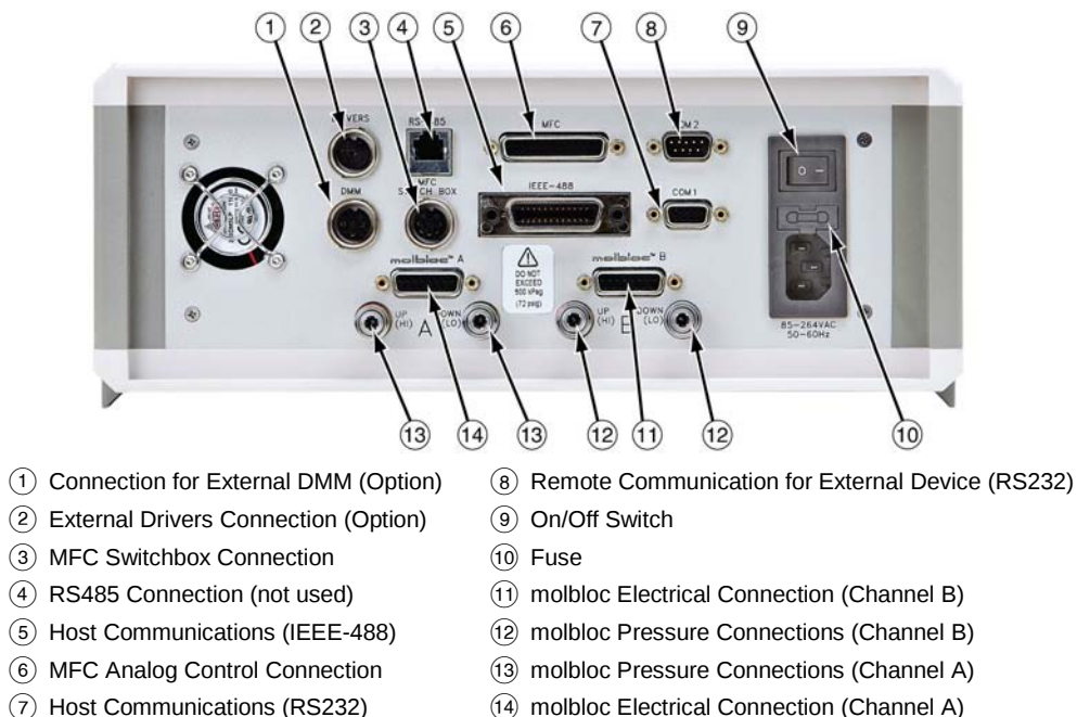
Figure 3. Rear Panel
