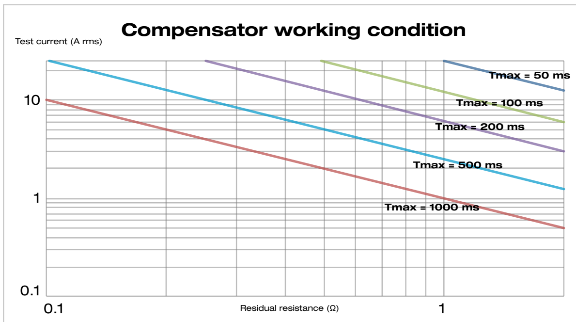
Residual resistance is the value of resistance which the Compensator can correct for based on the test current level sourced by the device under test (DUT). The T max parameter is the maximum time the compensator can correct the residual resistance before an overload condition is detected.
