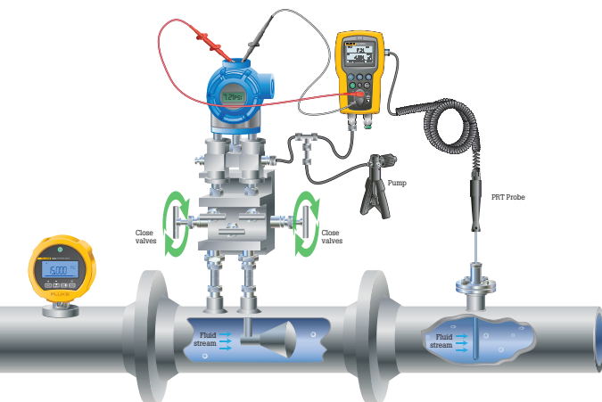
Figure 2. Sample flow transmitter with calibration equipment attached.
